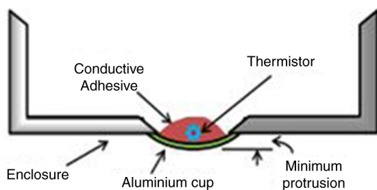
Figure 4 (A) Disassembled prototype; (B) vertical cross-sectional view of enclosure.
