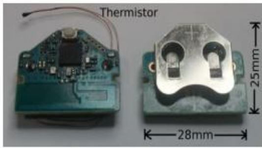
Web figure 2. Top and bottom view of the sensor
