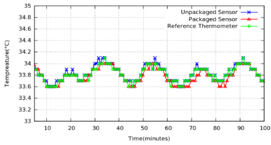
(b) Temp. measurements with hot plate at 34°C
