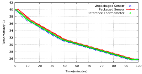
(c) Temperature measurements without hot plate
