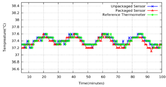
(a) Temp. measurements with hot plate at 37°C
